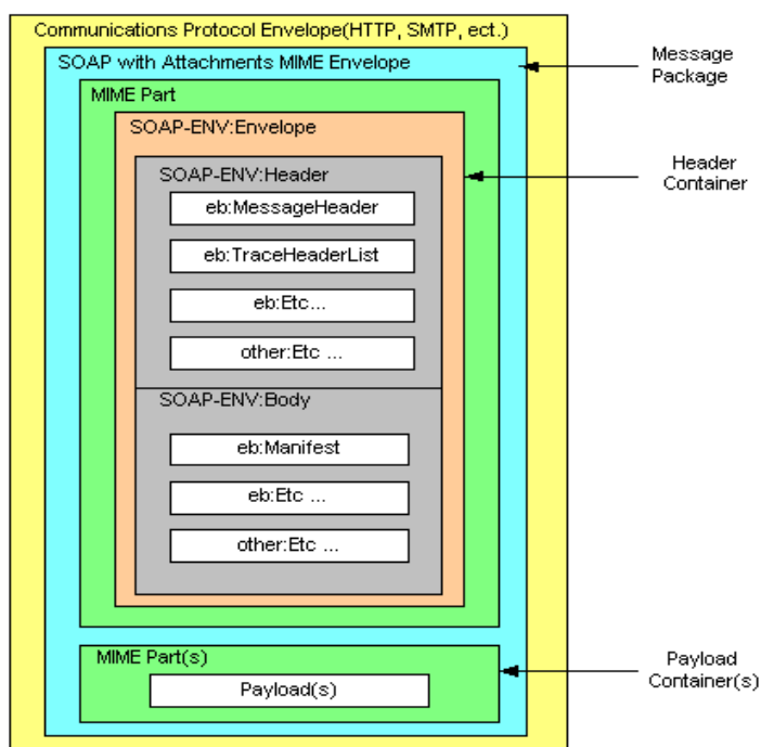
Figure 17 ebXML Message Structure and Composition
