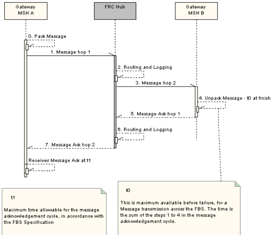
Figure 7 Timing steps in the Message cycle
