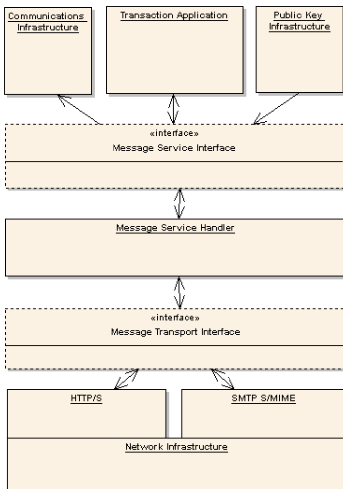
Figure 2 Logical Component View
