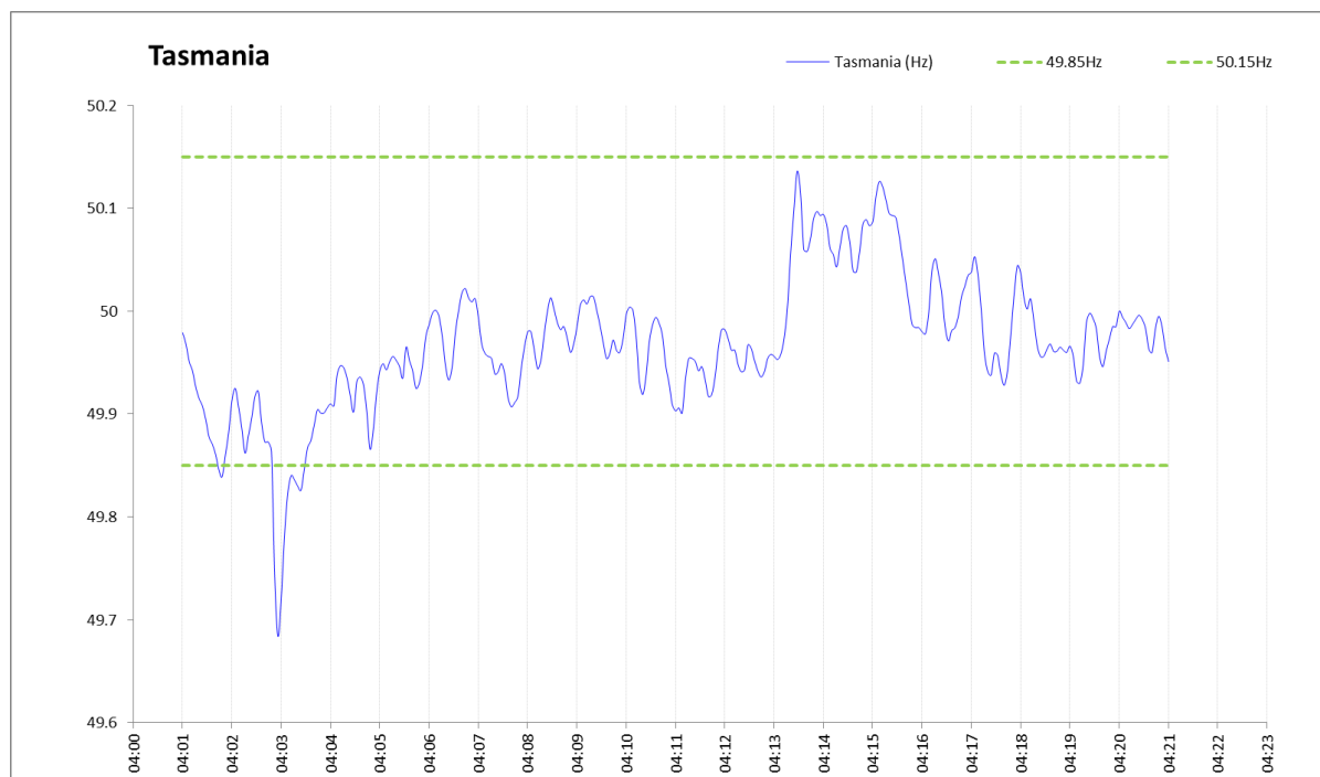
Figure 2: Low frequency event that occurred in Tasmania 0403 hrs 15 April 2013.
