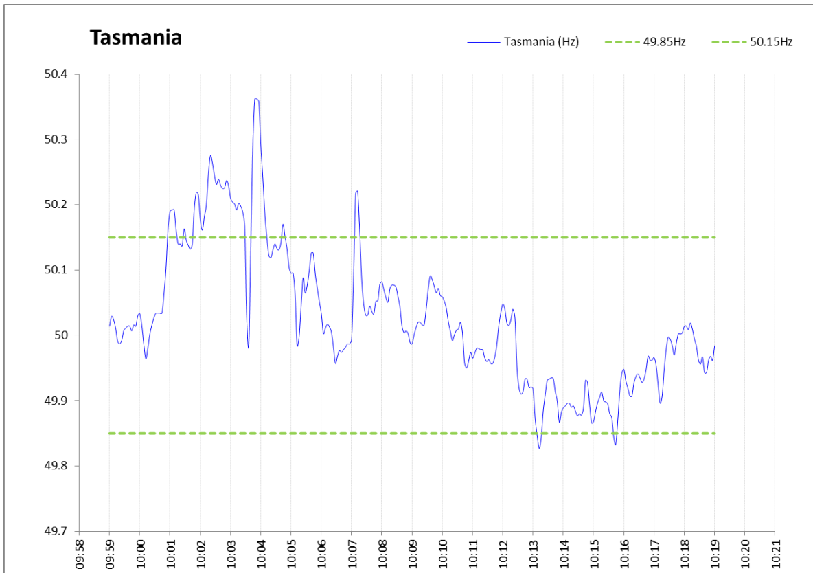
Figure 3: High frequency event that occurred in Tasmania 1001 hrs 15 April 2013.
