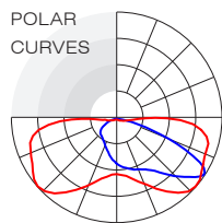
SATURN - P FORWARD THROW DISTRIBUTION Incremental tilting feature
