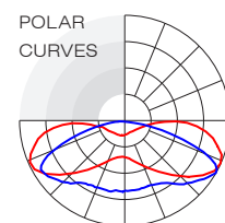
SATURN - A STREETLIGHT SIDE THROW DISTRIBUTION
