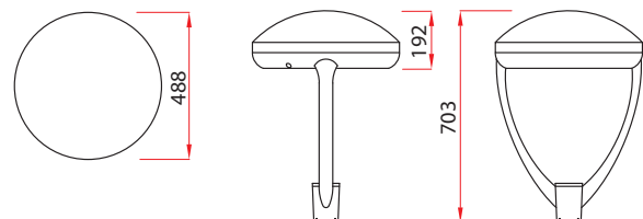
SATURN - A STREETLIGHT SIDE THROW DISTRIBUTION
